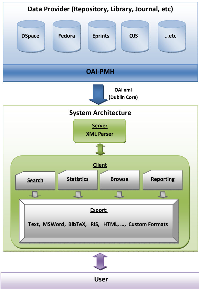
Figure 1. Architecture of value-added service implementation.
