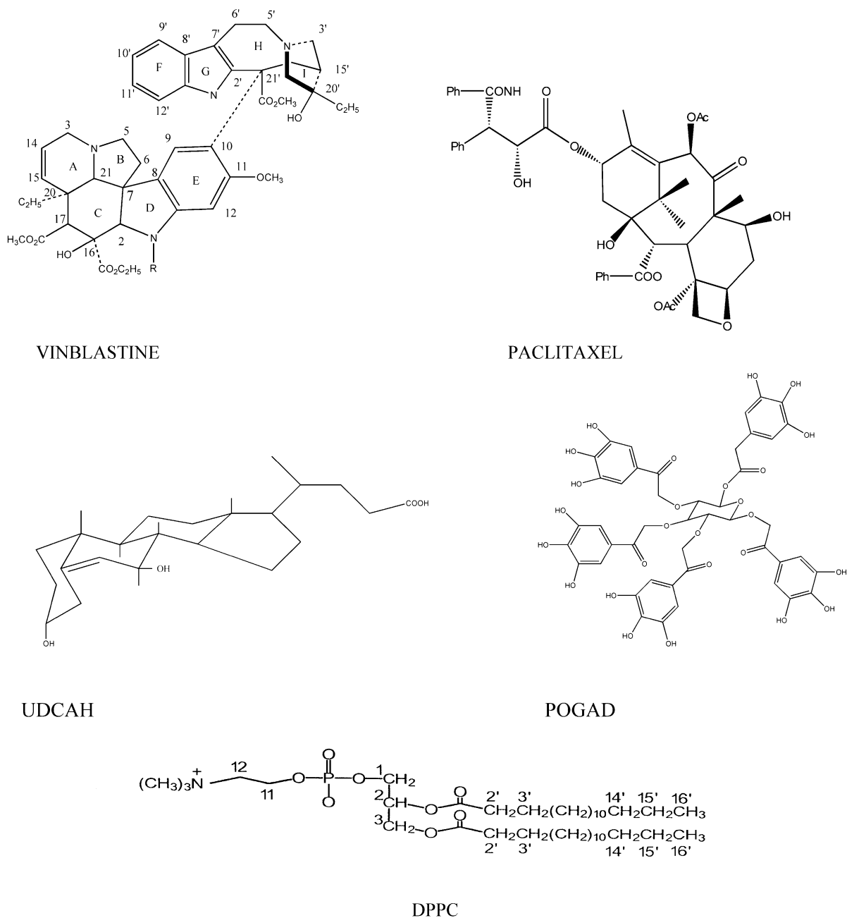
Fig. 1. Chemical structures of DPPC, vinblastine, UDCAH, paclitaxel, and penta- O -galloyl- \alpha -D-glucose.
