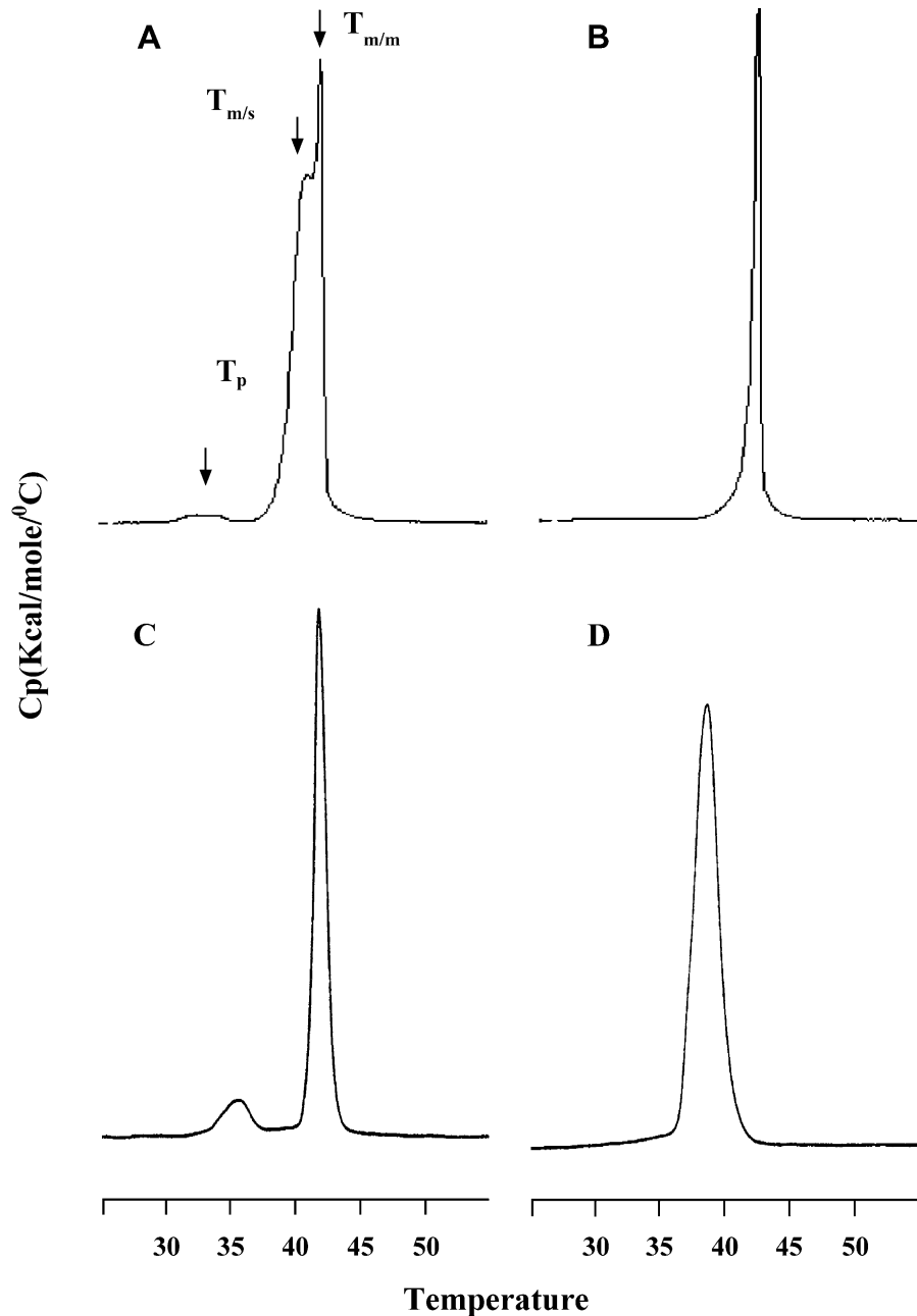
Fig. 2. (A, C) C_p vs. T data for a mixture of single- and multiple bilayer DPPC vesicles; T_{pu} and T_{pm} are the L'_\beta to P'_\beta pretransition temperatures for the uni- and multibilayer systems. Accordingly, T_{mu} and T_{mm} are the temperatures for the main-lipid phase transition of the two systems. (B, D) C_p vs. T data for the same mixture as in (A), with vinblastine sulfate incorporated in the DPPC membranes at molar concentration x=0.17 .
