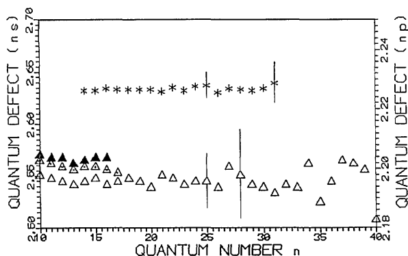
Fig. 3. Quantum-defect plots as a function of the quantum number n . Asterisks, 4sns series (left vertical axis); filled triangles, ^3P_0 levels; triangles with dots, ^3P_1 levels; open triangles, ^3P_2 levels of the 4snp series (right vertical axis). The error bars are according to Eq. (1) for \Delta E = 0.2 \text{ cm}^{-1} (experimental accuracy).
