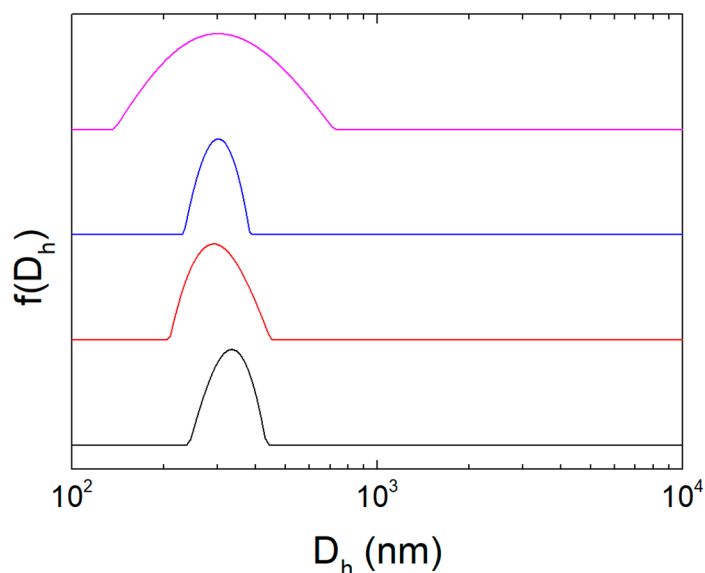
Figure 1. Size distributions of the dispersions from DLS on the day of preparation in HPLC grade water at 25\ ^\circ\text{C} and in PBS at 37\ ^\circ\text{C} . The line colors represent the different samples/conditions: sample 1 in HPLC grade water at 25\ ^\circ\text{C} (black), sample 2 in HPLC grade water at 25\ ^\circ\text{C} (red), sample 1 in PBS at 37\ ^\circ\text{C} (blue), and sample 2 in PBS at 37\ ^\circ\text{C} (magenta).
