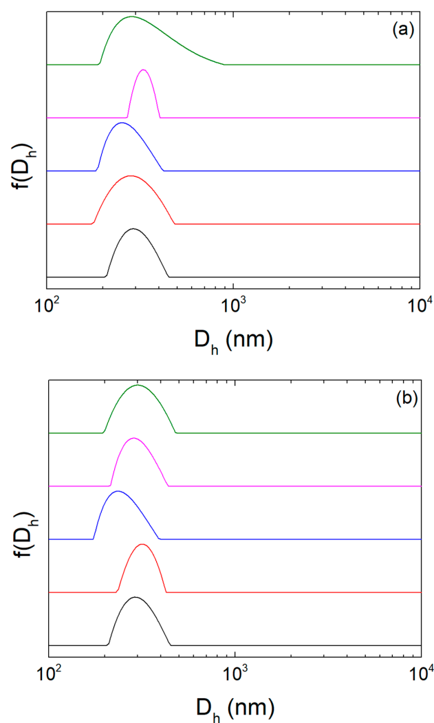
Figure 3. Size distributions of sample 2 from DLS under different storage conditions: (a) 25 °C and (b) 4 °C. The colors represent different time points from preparation T (days): T = 0 (black line), T = 1 (red line), T = 2 (blue line), T = 7 (magenta line), T = 9 (green line).
