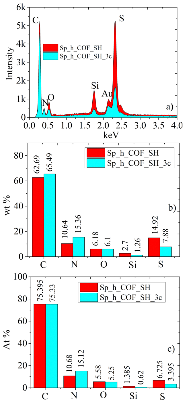
Fig. 5 (a) Representative EDS spectra of the thiol-modified sponges before (Sp_h_COFSH) and after 3 cycles of oil removal (Sp_h_COFSH_3c) and their wt% (b); at% (c). The data in (b) and (c) are the average of two different regions.
