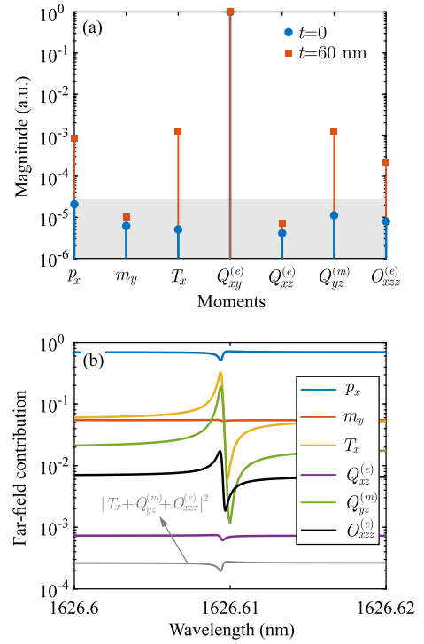
Fig. 7. Multipolar expansion analysis showcasing the transformation of the mode D_4 from BIC to qBIC, as the symmetry of the metasurface is reduced with the introduction of the silicon bridge. (a) Analysis with the eigenvector. The magnitude of the bright moments coupled to radiation fields polarized in the x direction is depicted, in the case of the symmetric (blue circles), and asymmetric (red squares) metasurface. The bright moments' magnitude are normalized with respect to the magnitude of the dominant dark moment Q_{xy}^{(e)} , which does not radiate in the far-field in the normal direction. The shaded area marks a practically zero level for the moments' magnitude. (b) Normalized far-field contribution of each bright moment individually in the scattered field as a function of the wavelength, when the metasurface is vertically illuminated by a plane wave polarized in the x direction.
