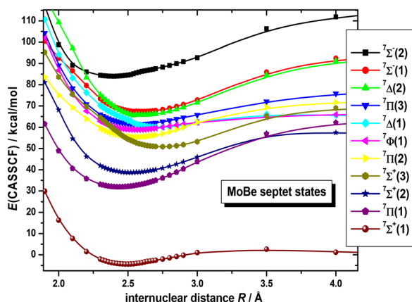
Fig. 3 Potential energy curves (PECs) of eleven septet states of MoBe at the SA-CASSCF/aug-cc-pV5Z(-PP) computational level. The \text{Mo}(a^7\text{S}) + \text{Be}(^4\text{S}) limit, to which the ^7\Sigma^+(1) state correlates, is used to define the zero of energy.
