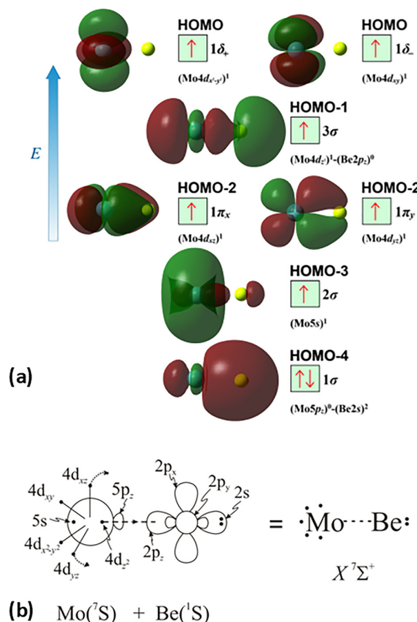
Scheme 1 (a) MOs diagrams and (b) valence bond Lewis diagram of the ground state X^7\Sigma^+ of \text{MoBe} at the CASSCF/aug-cc-pV5Z(-PP) level.
