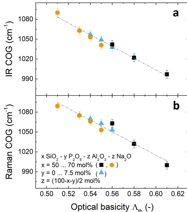
Fig. 7 Position of the centre of gravity (COG) of the high frequency envelope of IR (a) and Raman spectra (b) with respect to the optical basicity of the studied glasses. Blue triangles: 60 mol% \text{SiO}_2 and varying \text{P}_2\text{O}_5 content. Black squares: 0 mol% \text{P}_2\text{O}_5 and varying \text{SiO}_2 content. Orange circles: 7.5 mol% \text{P}_2\text{O}_5 and varying \text{SiO}_2 content. (Lines are linear fits. R^2 values are 0.976 for IR and 0.946 for Raman data.)
