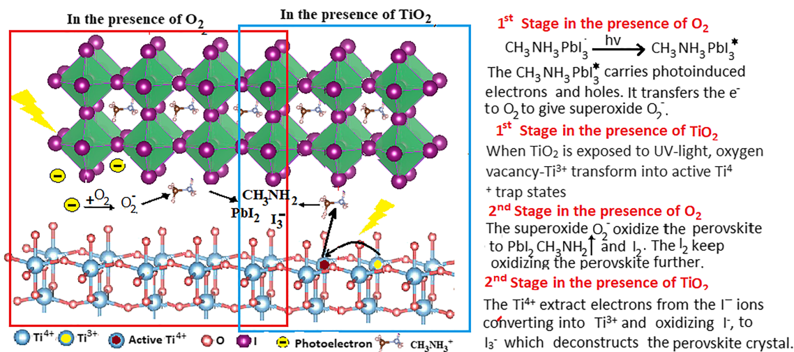
FIGURE 13 The mechanism of MHP degradation under continuous UV radiation in the presence of \text{O}_2 and/or \text{TiO}_2
