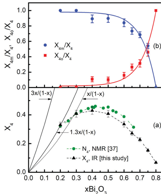
Fig. 8 (a) Comparison of the molar fractions of borate tetrahedral units in glasses xBi_2O_3-(1-x)B_2O_3 obtained in the present IR study, X_4 ( \blacktriangle ), and in the NMR study of ref. 37, N_4 ( \bullet ). Dashed lines are drawn as guides to the eye. The solid black lines present the theoretical value for the fraction of BO_4^- units, N_{4th} , formed at rates 3x/(1-x) , 1.3x/(1-x) and x/(1-x) . (b) Fractional contributions of the meta -borate tetrahedral units BO_4^- , X_{4m}/X_4 , and of the ortho -borate tetrahedral units BO_2O_2^{3-} , X_{4o}/X_4 , to the total fraction X_4 of borate tetrahedra in glasses xBi_2O_3-(1-x)B_2O_3 . Solid lines are the fitted exponential curves according to eqn (20).
