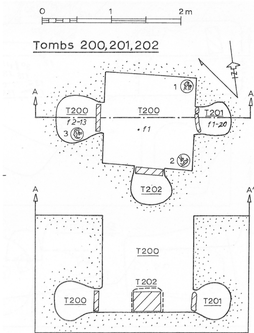
Fig. 1. Plan and section of pit-cave Tomb 200-202 at the site of Knossos Medical Faculty (after: Coldstream, Catling 1996e, fig. 43). Reproduced with permission of the British School at Athens.
