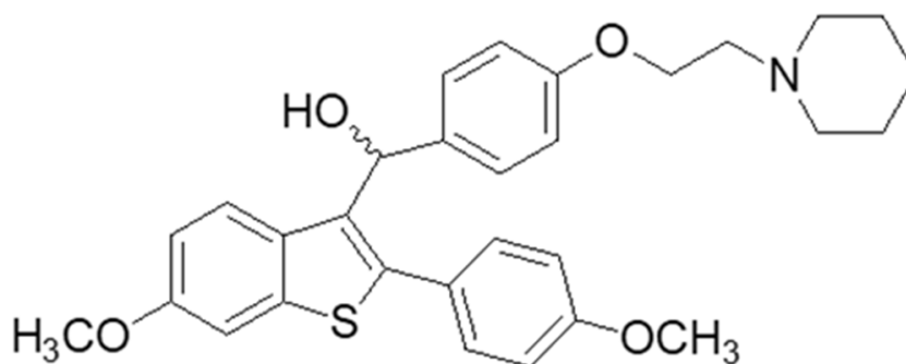
Figure 1. Chemical structure of DPS-2.
