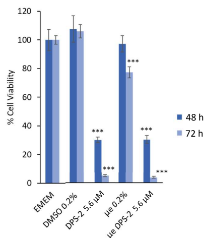
Figure 2. Inhibition of cell proliferation in SK-MEL 28 cells 48 and 72 h after the treatment onset. Culture medium (EMEM) and DMSO 0.2% v/v were used as positive control samples, \mu\text{e} 0.2% refers to O/W microemulsions without DPS-2 (empty), \mu\text{e} DPS-2 5.6 \mu\text{M} refers to O/W microemulsions loaded with DPS-2 at a concentration of 5.6 \mu\text{M} . DPS-2 was also solubilized in DMSO at 5.6 \mu\text{M} . Statistically significant results are indicated by asterisks (***) when p < 0.001 (Student's t -test).
