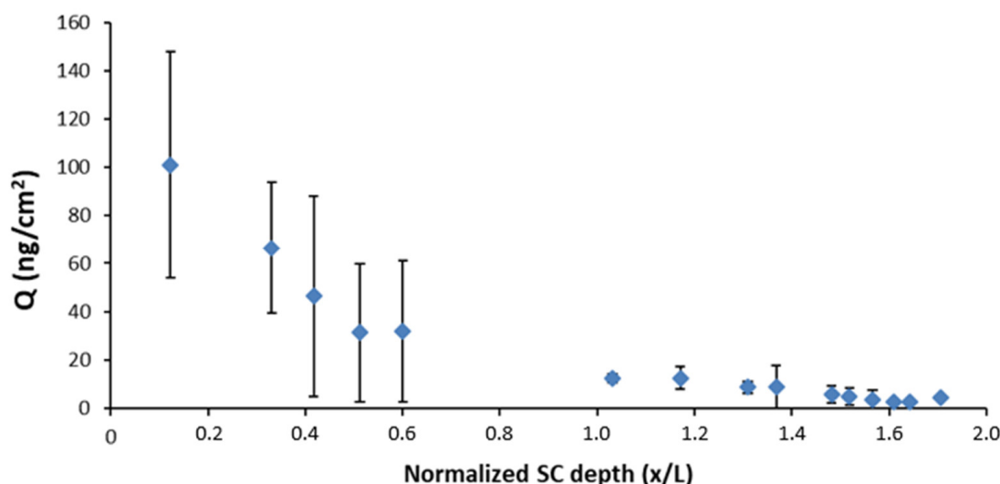
Figure 6. Representation of the quantity of DPS-2 ( \text{ng}/\text{cm}^2 ) in relation to the normalized SC depth.
