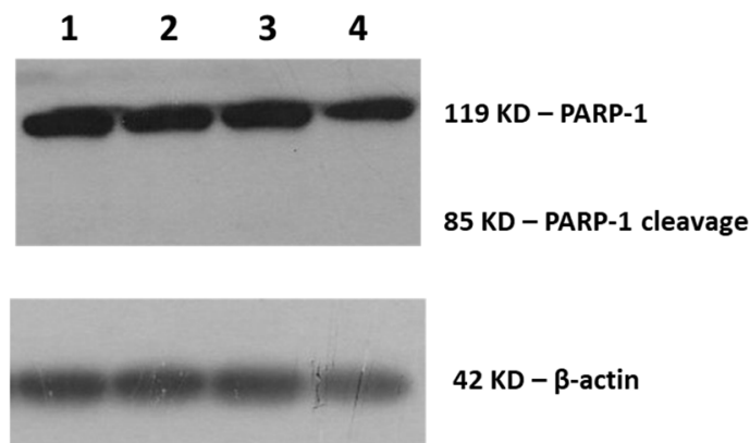
Figure 4. Cleavage of poly(adenosine diphosphate-ribose) polymerase 1 (PARP-1) for the assessment of cell death. Immunoblot of SK-MEL 28 cell extracts (25 \mu g) with anti-PARP-1 antibody detecting the 85 kDa PARP fragment (cleav. PARP-1) and the 119 kDa intact PARP-1 form. Cells were either not treated (EMEM-1) (1), treated with DPS-2 solubilized in DMSO at 5.6 \mu M (2), or treated with O/W microemulsion empty 0.2% v/v (3) or O/W microemulsion loaded with DPS-2 at 5.6 \mu M (4) and maintained in culture for 72 h. The relative abundance of the total protein applied was measured by using the amount of actin as a control, as assessed by the anti- \beta -actin on the same blot.
