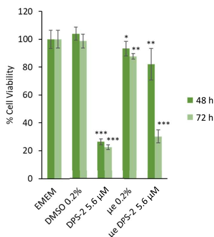
Figure 3. Inhibition of cell proliferation in WS1 cells 48 and 72 h after the treatment onset. Culture medium (EMEM) and DMSO 0.2% v/v were used as positive control samples, \mu\text{e} 0.2% refers to O/W microemulsions without DPS-2 (empty), \mu\text{e} DPS-2 5.6 \mu\text{M} refers to O/W microemulsions loaded with DPS-2 at a concentration of 5.6 \mu\text{M} . DPS-2 was also solubilized in DMSO at 5.6 \mu\text{M} . Statistically significant results are indicated by asterisks (*) when p < 0.05 , (**) when p < 0.01 , and (***) when p < 0.001 (Student's t -test).
