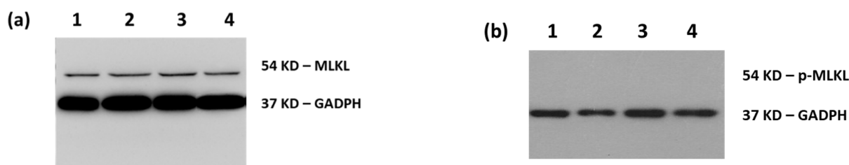
Figure 5. Immunodetection of necroptotic cell death markers. Phosphorylation of mixed lineage kinase domain-like protein (MLKL) at ser358. Immunoblot of SK-MEL 28 cell extracts (25 \mu g) with (a) anti-MLKL antibody detecting all forms of the MLKL protein (54 kDa) and (b) anti-phospho-MLKL antibody detecting the phosphorylation of MLKL at serine 358 (54 kDa) upon the activation of necroptosis. Cells were either not treated (EMEM-1) (1), treated with DPS-2 solubilized in DMSO at 5.6 \mu M (2), or treated with O/W microemulsion empty 0.2% v/v (3) or O/W microemulsion loaded with DPS-2 at 5.6 \mu M (4) and maintained in culture for 72 h. The relative abundance of total protein applied was measured by using the amount of GAPDH as a control, as assessed by the anti-GAPDH on the same blot.
